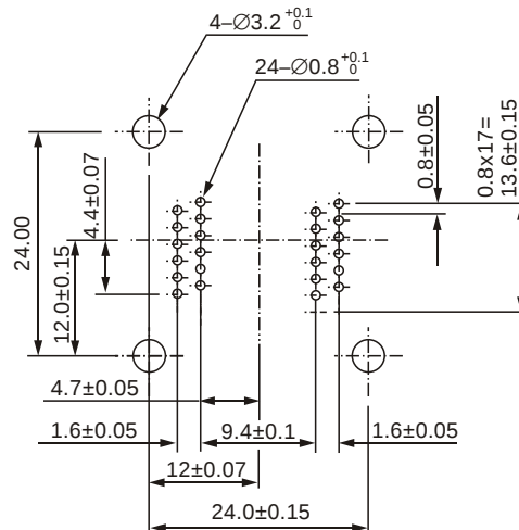
24 pins (SOP)
