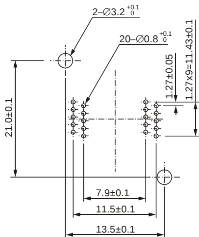
20 pins (SOP)
